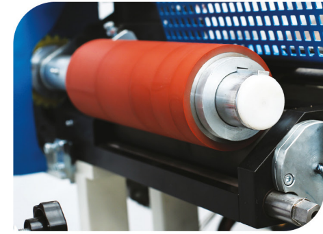
Özel Olarak Tasarlanmış PP, Finish Folyo, Doğal Kaplama ve Laminat Malzemelerine Tutkal Uygulayan Merdane Glue Application Roller is Designed for special production of PP, Finish Folio, Natural Coating and Lamination
